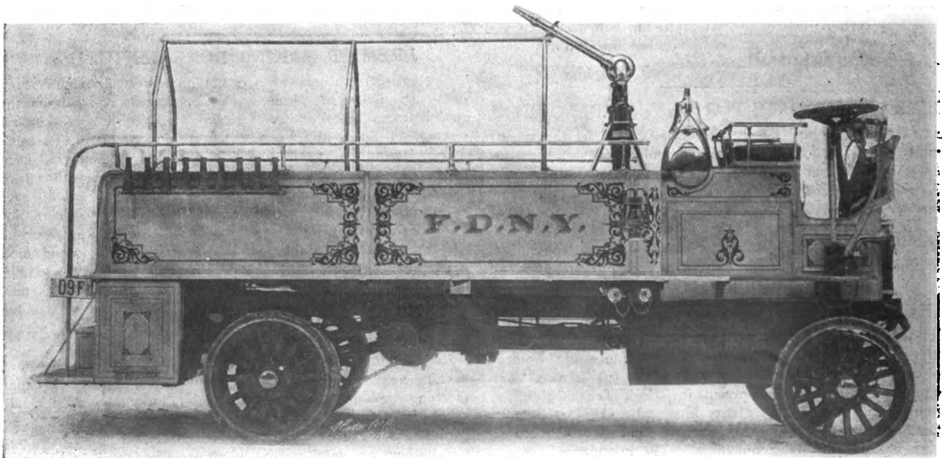
High-Pressure Hose Wagon Built for the Fire Department of New York City, by Knox Automobile Company.
